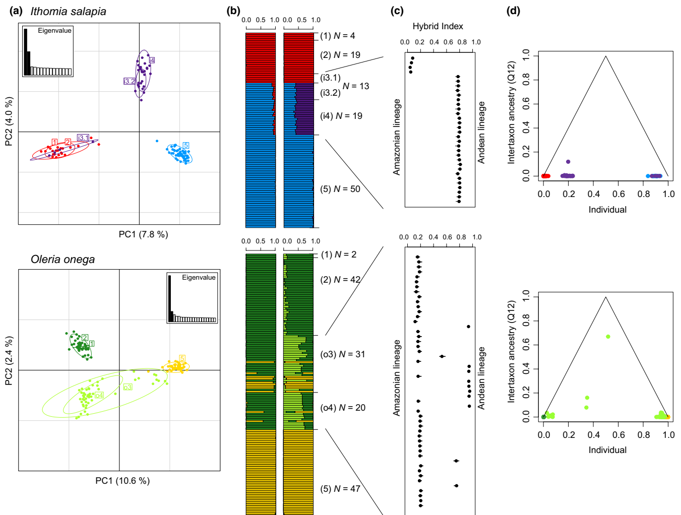
FIGURE 2 Population structure of pure and hybrid populations of Ithomia salapia (top) and Oleria onega (bottom). (a) Principal component analysis (PC1: horizontal axis, PC2: vertical axis), the percentage of total inertia explained by each axis is indicated in parentheses and the histograms in the top corners represent the inertia percentages of the first principal components. (b) Structure plot for K = 2 and K = 3 . The number of individuals that were used is indicated for each site. (c) Plot of the hybrid index of each sample from the hybrid populations. The points represent the mean hybrid index value estimated from the posterior distribution and black lines indicate 95% credible intervals. (d) Plot of intertaxon ancestry and hybrid index. Population colour codes are the same as those in Figure 1b [Colour figure can be viewed at wileyonlinelibrary.com ]
