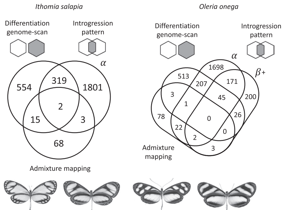
FIGURE 6 Venn diagram combining number of SNPs identified as supported by each approach (differentiation, introgression and admixture mapping) and shared between them. Note that for introgression patterns, no SNP showed deviant genomic cline rate parameters ( \beta ) in I. salapia . This parameter is therefore not represented in the diagram [Colour figure can be viewed at wileyonlinelibrary.com ]
