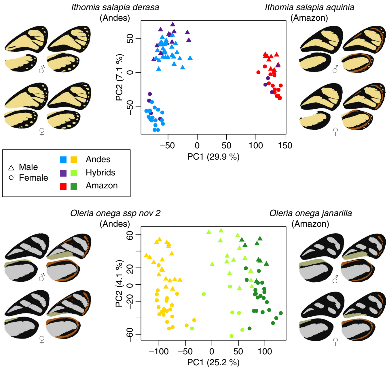
FIGURE 4 Phenotypic position of 90 I. salapia (top) and 94 O. onega (bottom) in the wing colour space consisting of the two main principal components from the colour pattern modelling approach. Colour indicates sample populations as in Figure 1b. Females and males are depicted by circles and triangles, respectively. Representative images of the average phenotypes for population and sex are shown on each side of the figure [Colour figure can be viewed at wileyonlinelibrary.com ]
