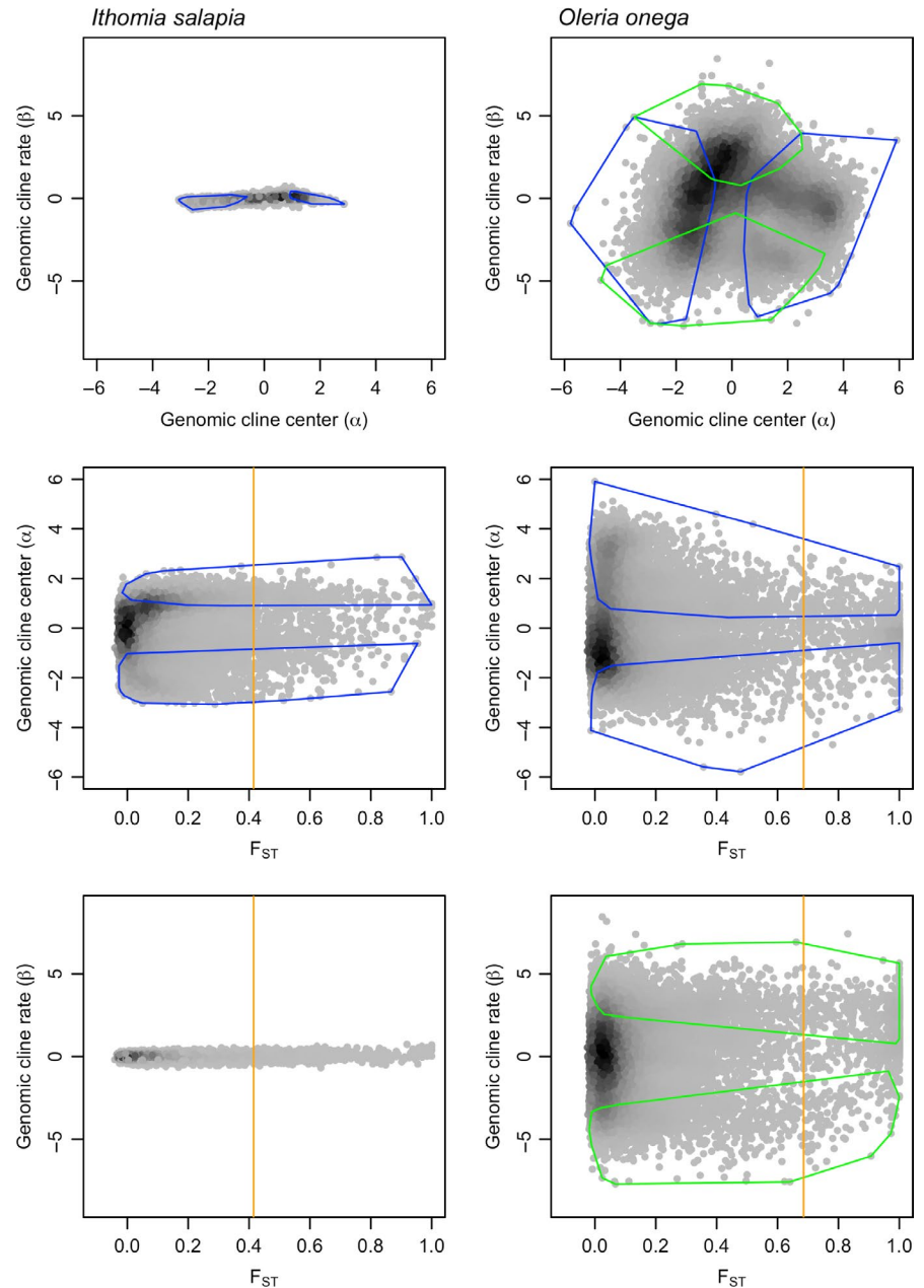
FIGURE 3 Scatterplots representing the relationships between the genomic cline center parameter ( \alpha ), representing SNP ancestry; the genomic cline rate parameter ( \beta ), representing the steepness of the cline; and the differentiation level, F_{ST} , estimated for each SNP. Plots for I. salapia and O. onega are on theft and right, respectively. Each data point is coloured in grey, and darkness increases with point density (i.e., darker areas contain more points). Blue lines frame sets of SNPs for which the genomic cline center parameters ( \alpha ) significantly deviates from the genome-wide pattern. Green lines frame sets of SNPs for which the genomic cline rate parameters ( \beta ) significantly deviates from the genome-wide pattern. Note that for I. salapia , no SNPs have genomic cline rate parameters ( \beta ) that deviate from the genome-wide pattern. SNPs on the right hand side of the orange lines harbour a significantly higher differentiation (high F_{ST} ) than the genome average [Colour figure can be viewed at wileyonlinelibrary.com ]
