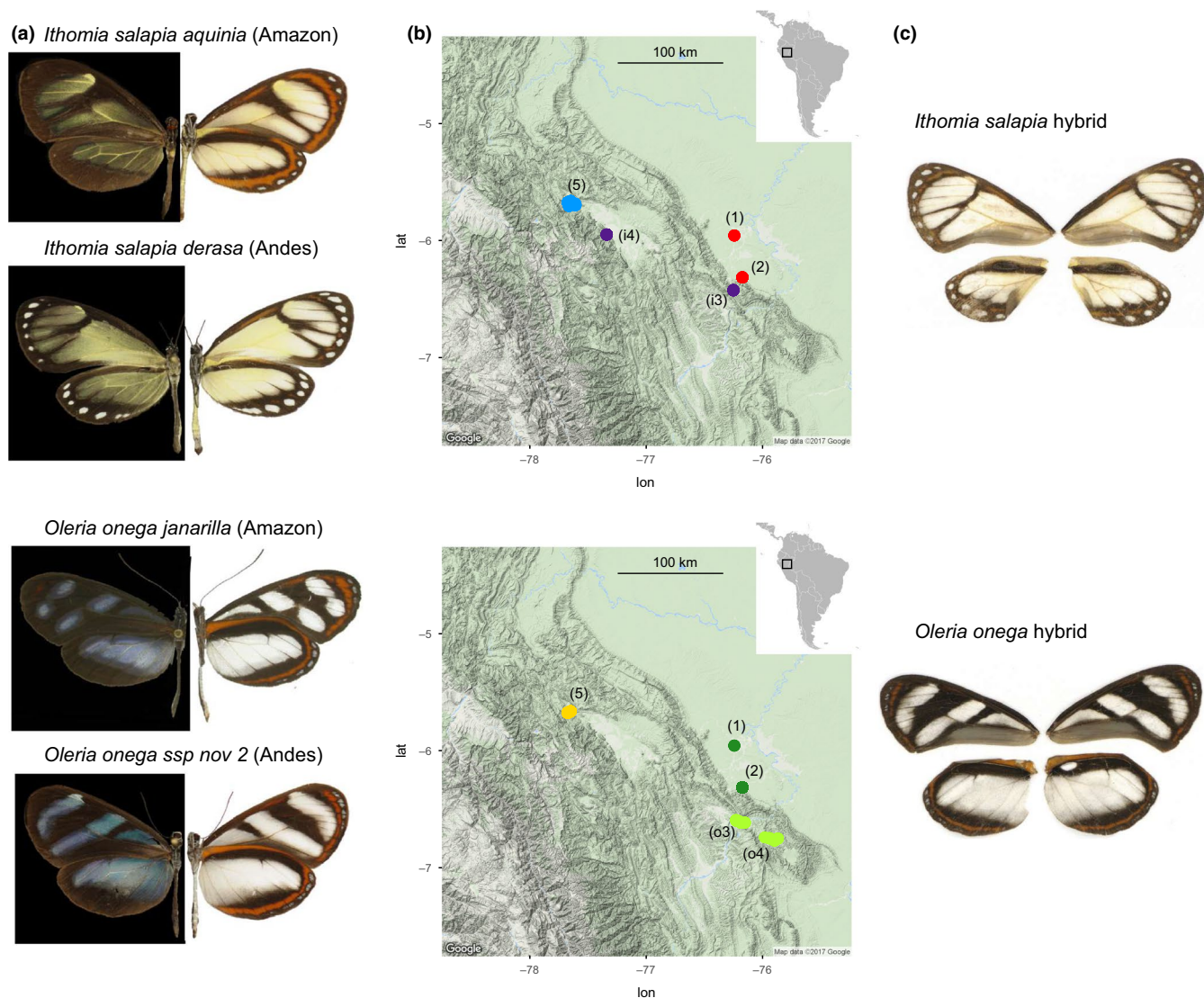
FIGURE 1 The study organisms and sites studied in N.E. Peru. (a) Photos of representative specimens from each population of the two studied species (dorsal side shown against a dark background to highlight transparency and ventral side shown against a white background to highlight colour pattern). (b) Sampling sites for I. salapia populations (top) with Amazonian sites in red (1) Km-26 Yurimaguas-Tarapoto and (2) San Miguel de Achinamiza, the Andean sites in blue (5) Puente Aguas Verdes and sites within the hybrid zone in purple (i3) Km-42 Tarapoto-Yurimaguas and (i4) La Florida. For O. onega populations (bottom), Amazonian sites are in green (1) Km-26 Yurimaguas-Tarapoto and (2) San Miguel de Achinamiza, Andean sites are in yellow (5) Puente Serranoyacu and the sites in the hybrid zone are in apple green (o3) Shapaja-Chazuta (o4) from Quebrada Yanayacu to Laguna del Mundo Perdido. Colour codes are conserved for all other figures. (c) Photographs of putative hybrid specimens with intermediate colour patterns (ventral side). Photograph credits: Céline Houssin [Colour figure can be viewed at wileyonlinelibrary.com ]
